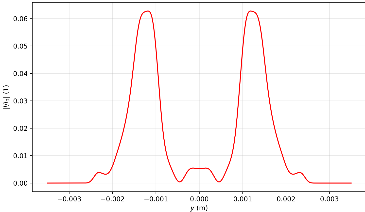
Intensity profile I(x=0, y, z=3.821)/I_0 , P_{in}=7.5P_{cr} , artificial time
